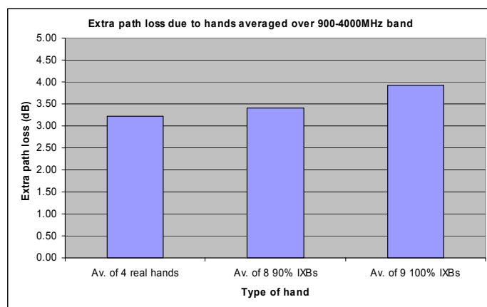
Average of extra path loss introduced by real hands compared to larger and smaller hands.
